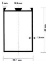
Lateral
