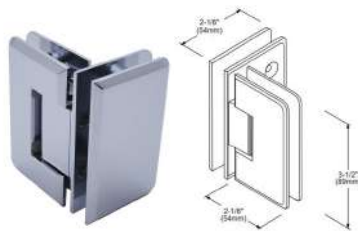
Bisagra V/V 90°
