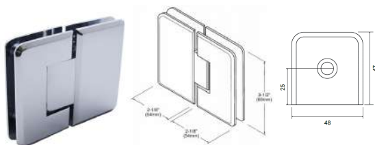
Conector V/V 180°
