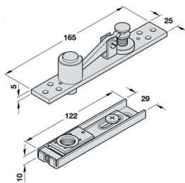
Pivote Ajustable
