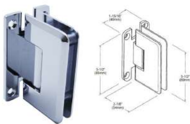
Bisagra P/V 90°
