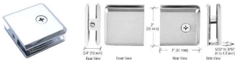
Conector P/V 90°
